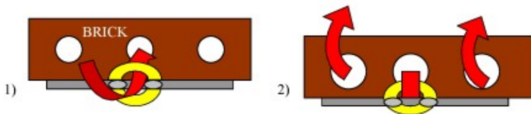
Figure B. Side views of brick attachment to PVC plate. Step D (left) and Step F (right)
